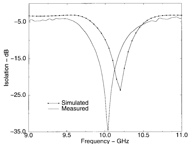
Fig. 19. Simulated and measured isolation between T/R ports of the antenna from Fig. 18.
