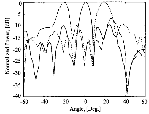
Fig. 16. Beam scanning in H -plane at 10.1 GHz for the 24-element lens amplifier array in receive mode. Receive horn at (—) 0^\circ , (---) -20^\circ , and (···) 20^\circ locations are shown. The normalizing power levels of the main lobes are within 2 dB.
