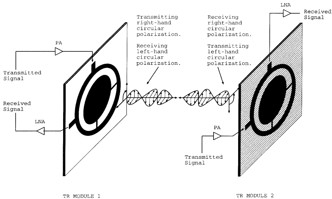
Fig. 18. Perspective view of a compact circularly polarized T/R antenna.
