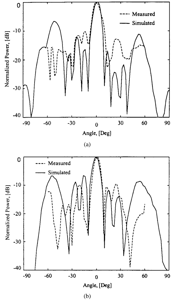
Fig. 9. (a) Measured (---) and simulated (—) E -plane radiation pattern for the receive amplifier at 10.1 GHz. (b) Measured (---) and simulated (—) H -plane radiation pattern for the receive amplifier at 10.1 GHz. The theoretical patterns were calculated for a uniform array using the measured antenna pattern of a single-slot antenna.
