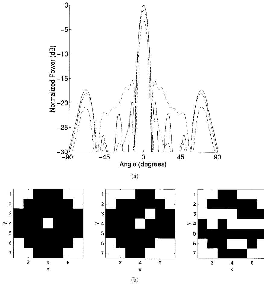
Fig. 20. (a) Simulated radiation pattern as 10% (dashed line) and 30% (dotted line) elements fail randomly across the Ka -band lens array from Section II-C. (b) The white blocks show which elements in the array are simulated as failed in the two cases. The solid line shows the antenna pattern of the fully functional array, with the white square in the middle indicating the feed element in the folded focus approach.
