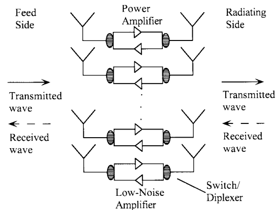
Fig. 1. A sketch of a general QO T/R analog front end.
