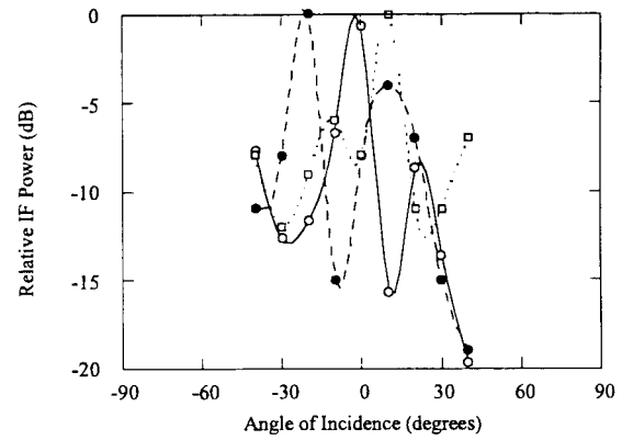
Fig. 13. Three received IF signals in a receiver with angle diversity. The three signals are measured at three mixers positioned along a focal arc, as a carrier source is moved in the far field [7].
