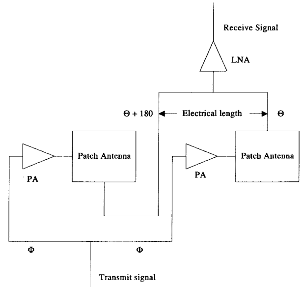
Fig. 17. A sequentially rotated two-element T/R array [14].
