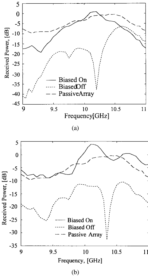
Fig. 8. (a) Measured ON/OFF ratio of the 24-element active and passive array in transmit mode, with polarizers at input and output. (b) Measured ON/OFF ratio of the 24-element active and passive array in receive mode, with polarizers at input and output. The measurements are normalized to a through measurement with a rectangular aperture surrounded by absorbing material. The solid lines represents the biased on state, the dotted lines the biased off state, and the dashed lines shows the measured results for the passive array.
