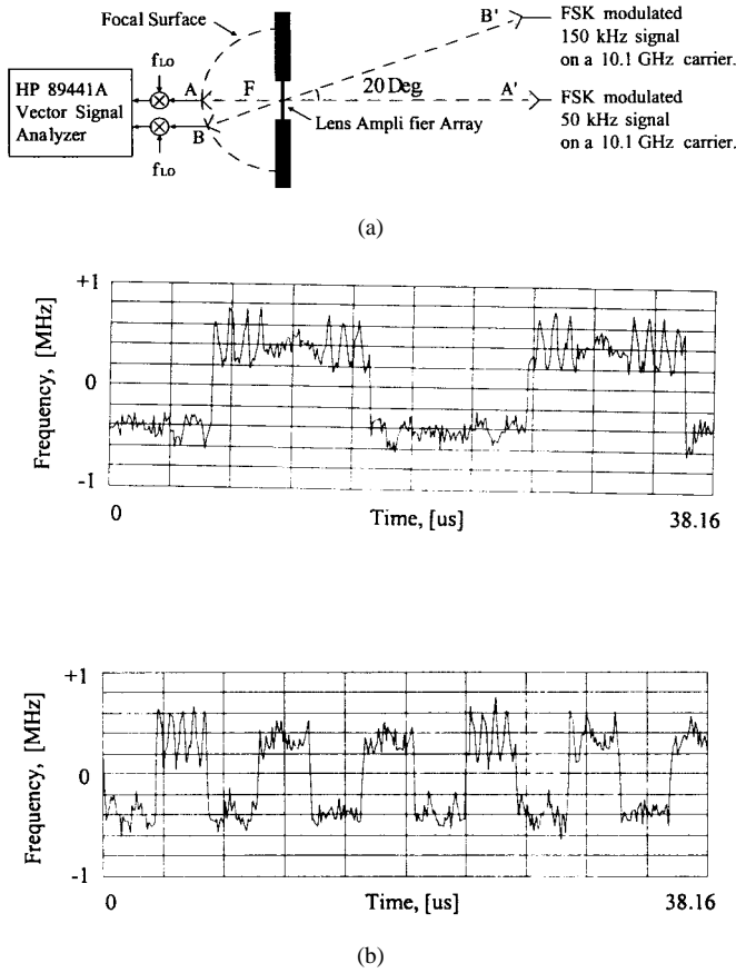
Fig. 15. (a) Test setup for the multiuser experiment. Square-wave signals at f_A = 50 kHz and f_B = 150 kHz are frequency modulated on a 10.1-GHz carrier and input at 0^\circ and 20^\circ from the optical axis, respectively. The two signals are received by horns located on the focal surface behind the 24-element lens amplifier array, and demodulated using a vector signal analyzer. (b) Received and frequency-shift keying (FSK) demodulated 50- and 150-kHz signals for receivers located at 0^\circ and 20^\circ , left and right, respectively.
