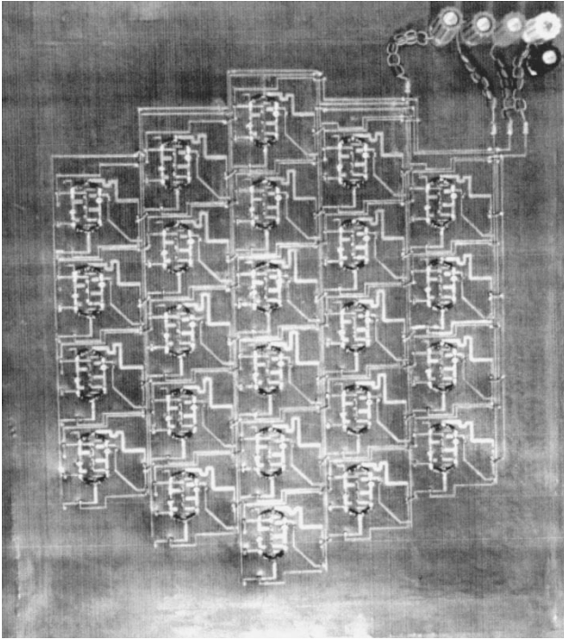
Fig. 6. (a) Unit cell of a slot-antenna T/R lens array. The slots are connected through transmit or receive paths by switching the p-i-n diodes. (b) Photograph of the circuit side of the 24-element bidirectional amplifier array. Orthogonally polarized slot antennas are located in the ground plane.
