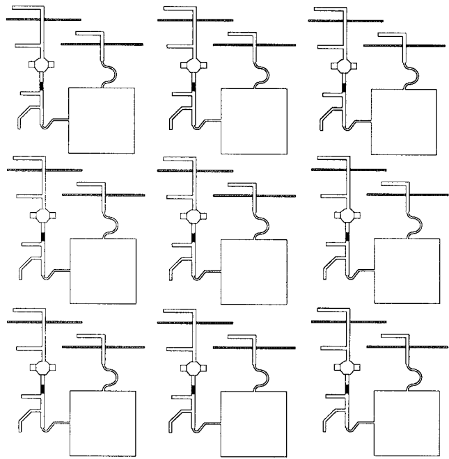
Fig. 3. Circuit layout of the 3 \times 3 X-band T/R array. Transmitting and receiving sides have symmetrical layouts.
