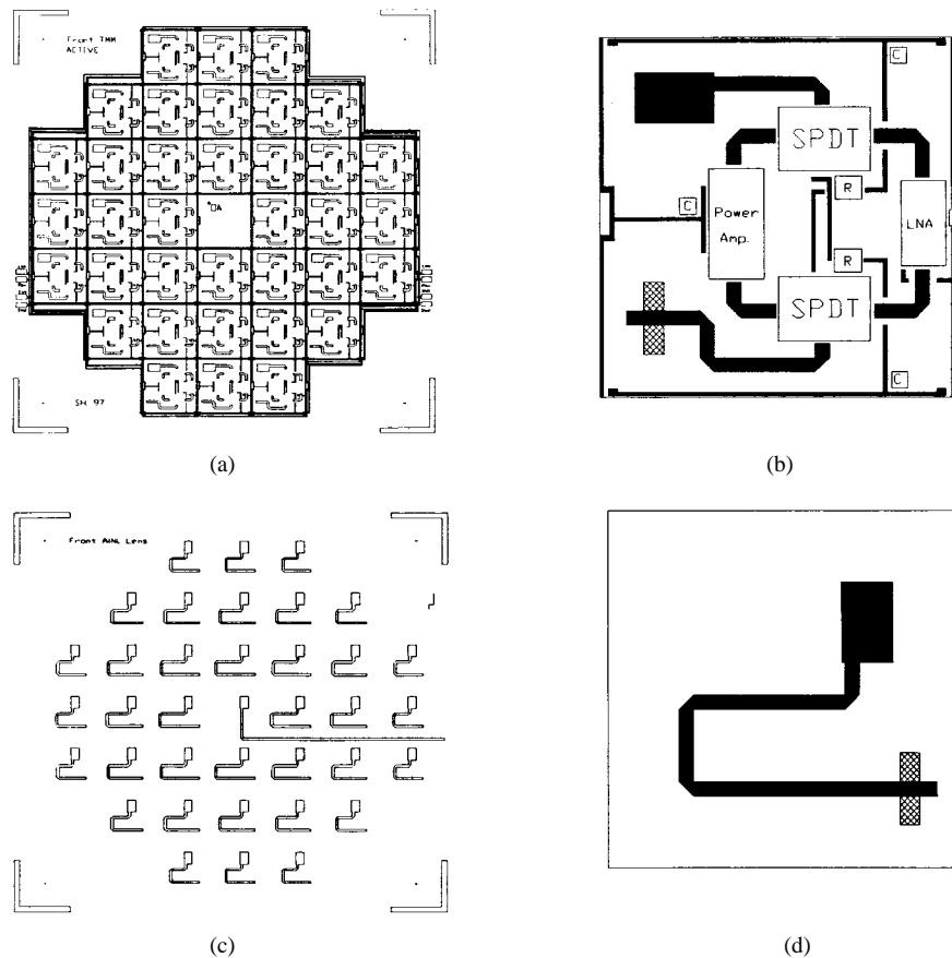
Fig. 10. (a)–(b) Front and (c)–(d) back sides of a patch-antenna hybrid Ka -band bidirectional lens amplifier array and unit cell. The unit-cell size is 1\lambda^2 .
