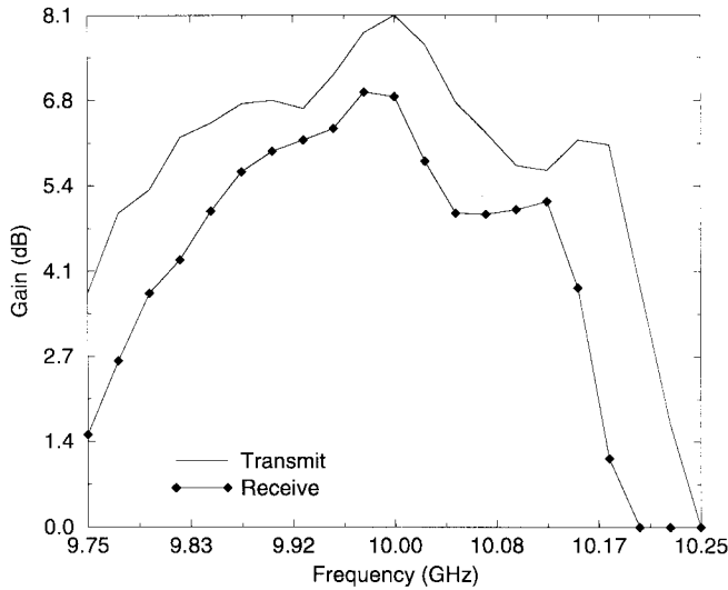
Fig. 4. T/R far-field gain measurements of the 3 \times 3 T/R array.
