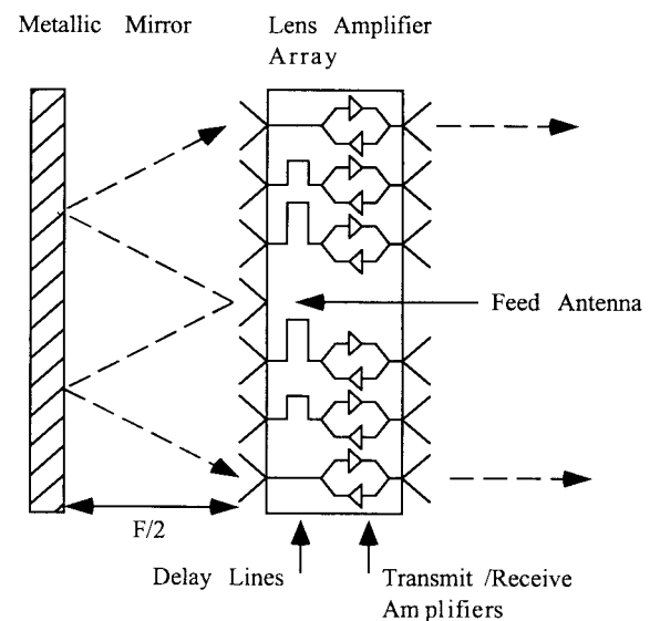
Fig. 11. “Folded” lens amplifier geometry. The lens is fed by its center elements, which does not contribute directly to the combined output power.
