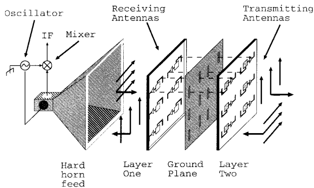
Fig. 2. Perspective view of a T/R double-layer X-band array.
