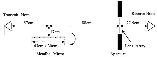
Fig. 7. Setup for measuring a lens amplifier bidirectional array. The translatable mirror is used only for a multipath reduction experiment, which is described in Section III.
